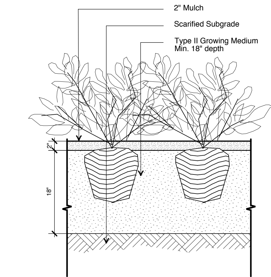
Ld - 03 Shrub Planting on Grade LWF 3.2 Scale 1" = 1'
