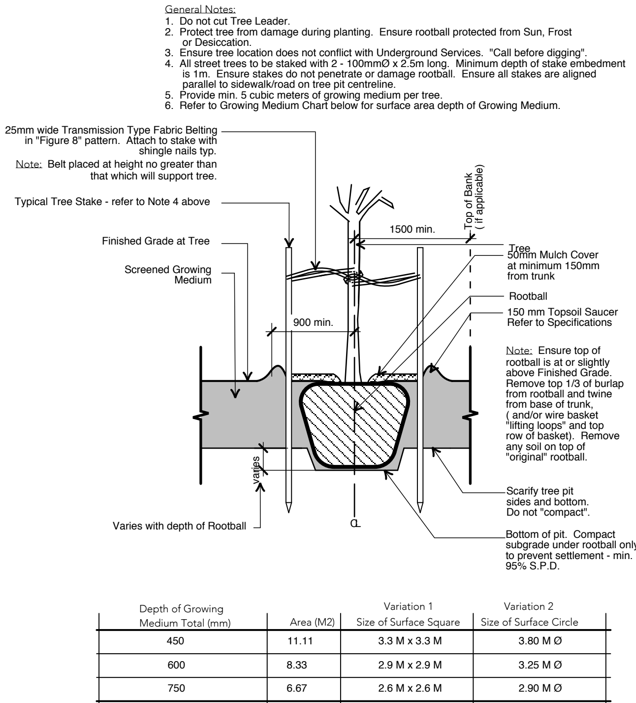
Ld - 01 Tree Planting on Grade LWF 3.2 Not to Scale
