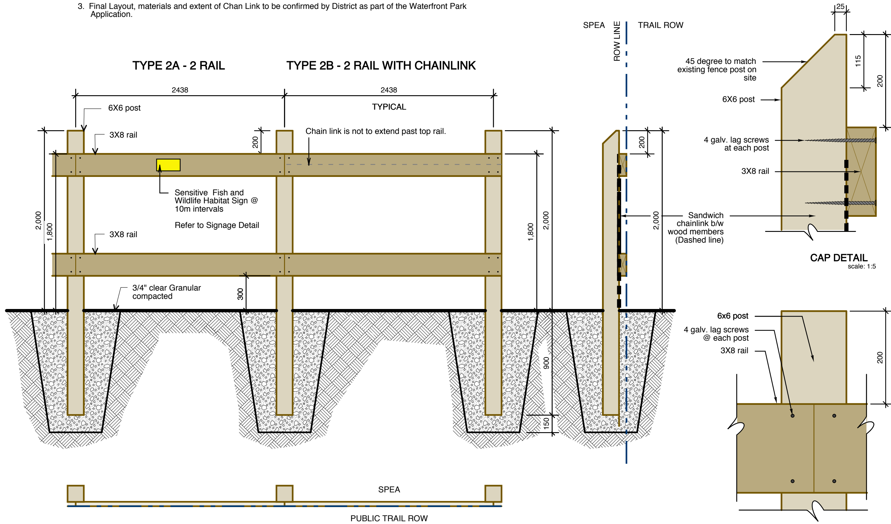
Ld - 04 Waterfront Park: Riparian Fence LWF 3.2 1:20
