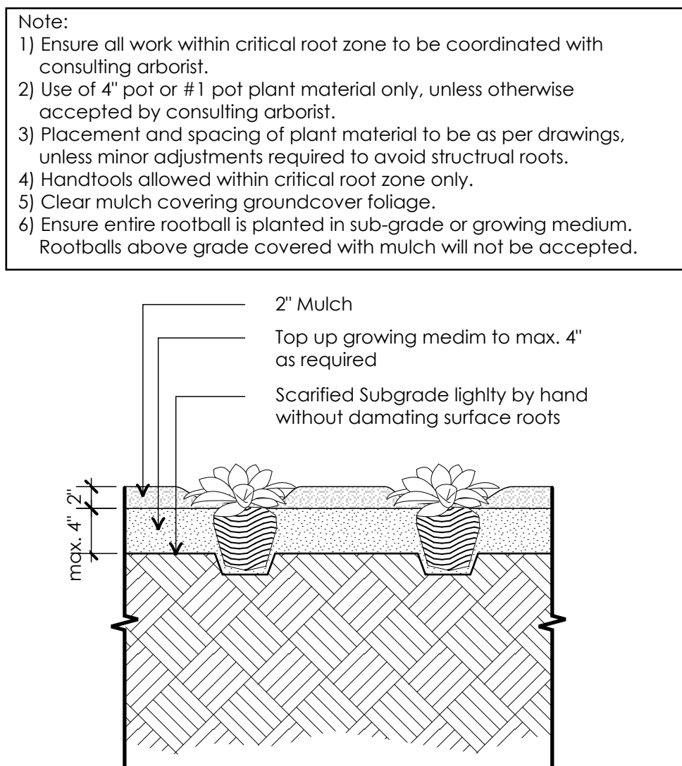
Ld - 02 Pocket Planting in Tree Protection Zone LWF 3.2 Scale 1" = 1'-0"
