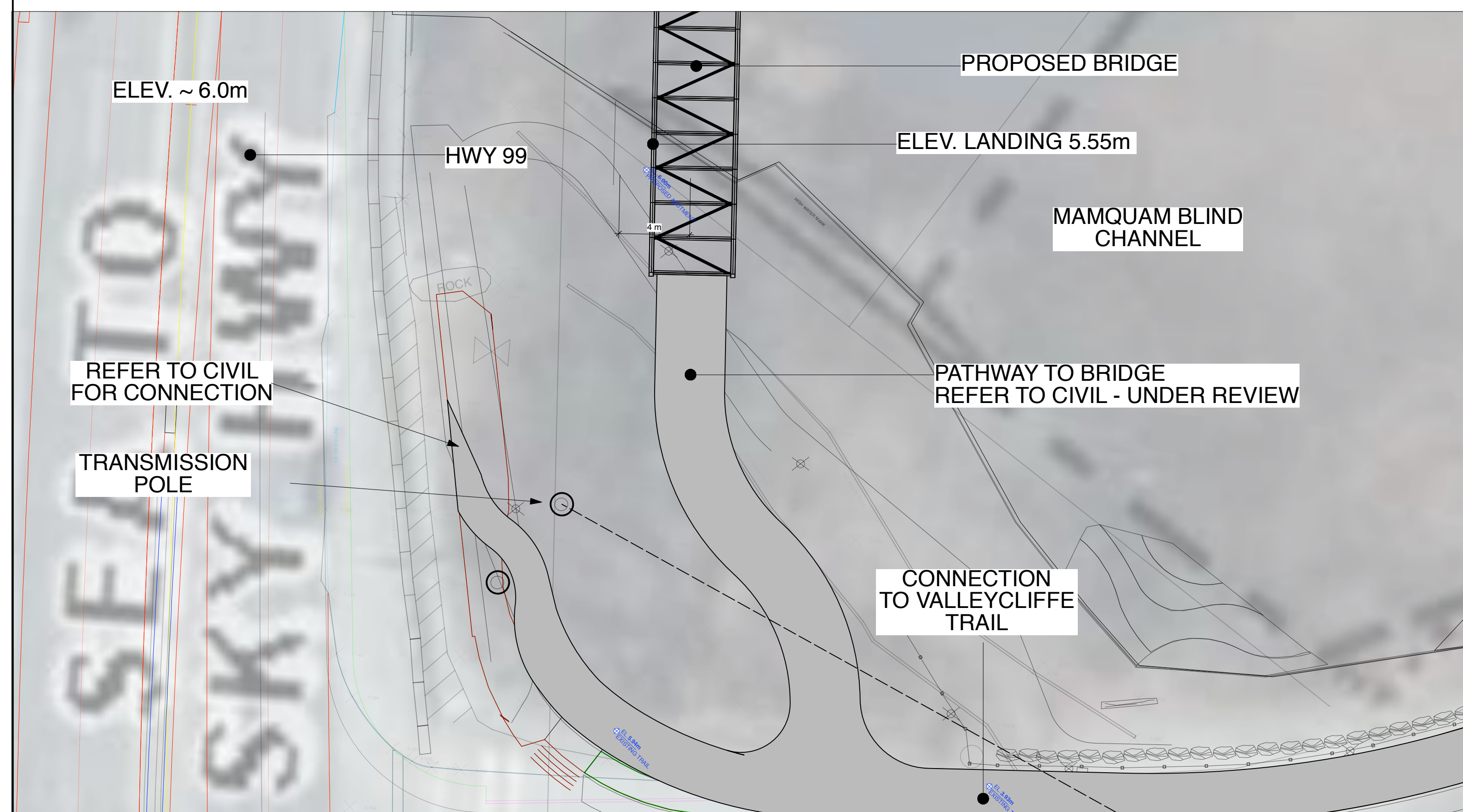
BRIDGE: NORTH LANDING Scale : 1:200
