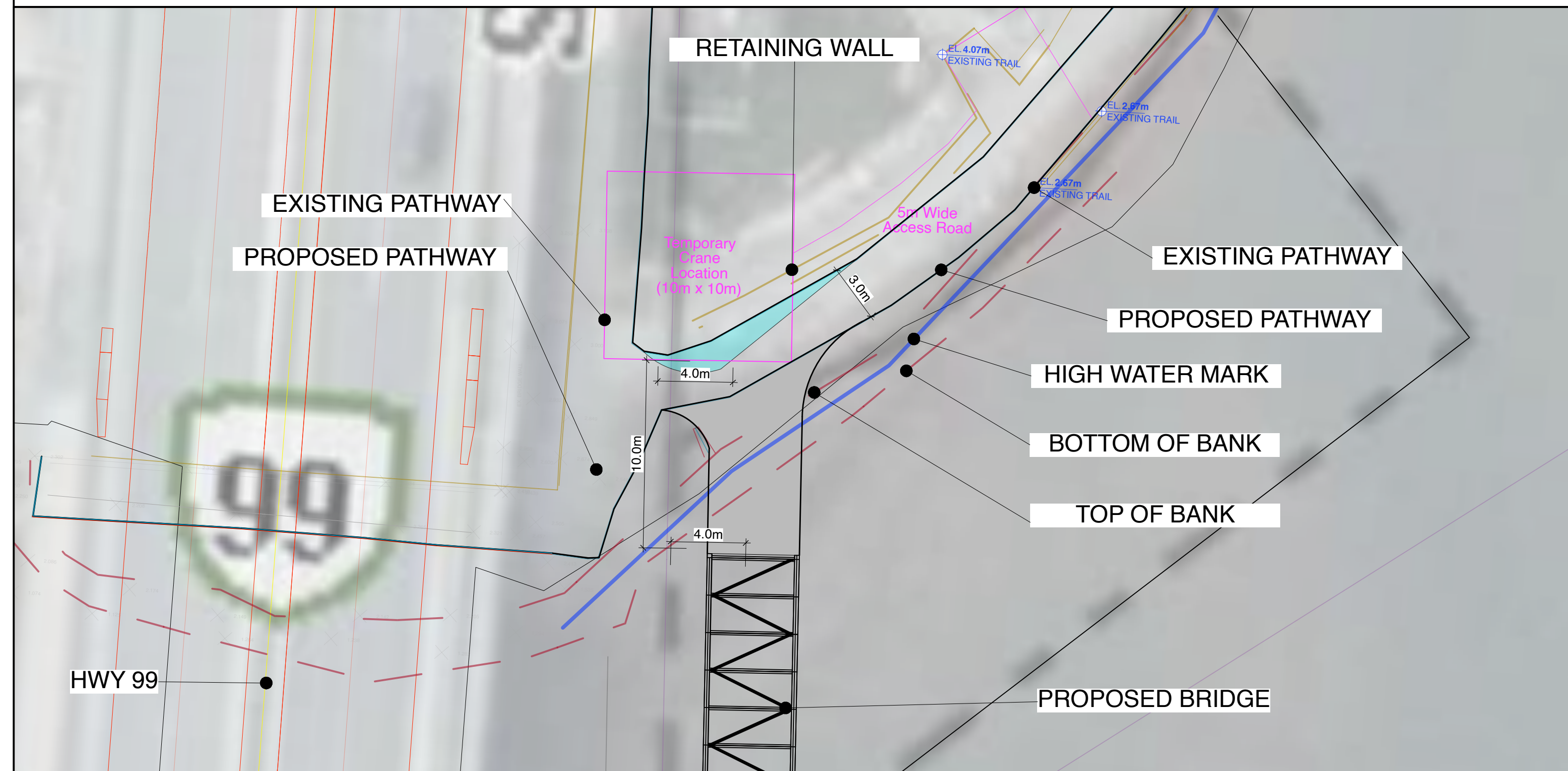
BRIDGE: NORTH LANDING Scale : 1:200
