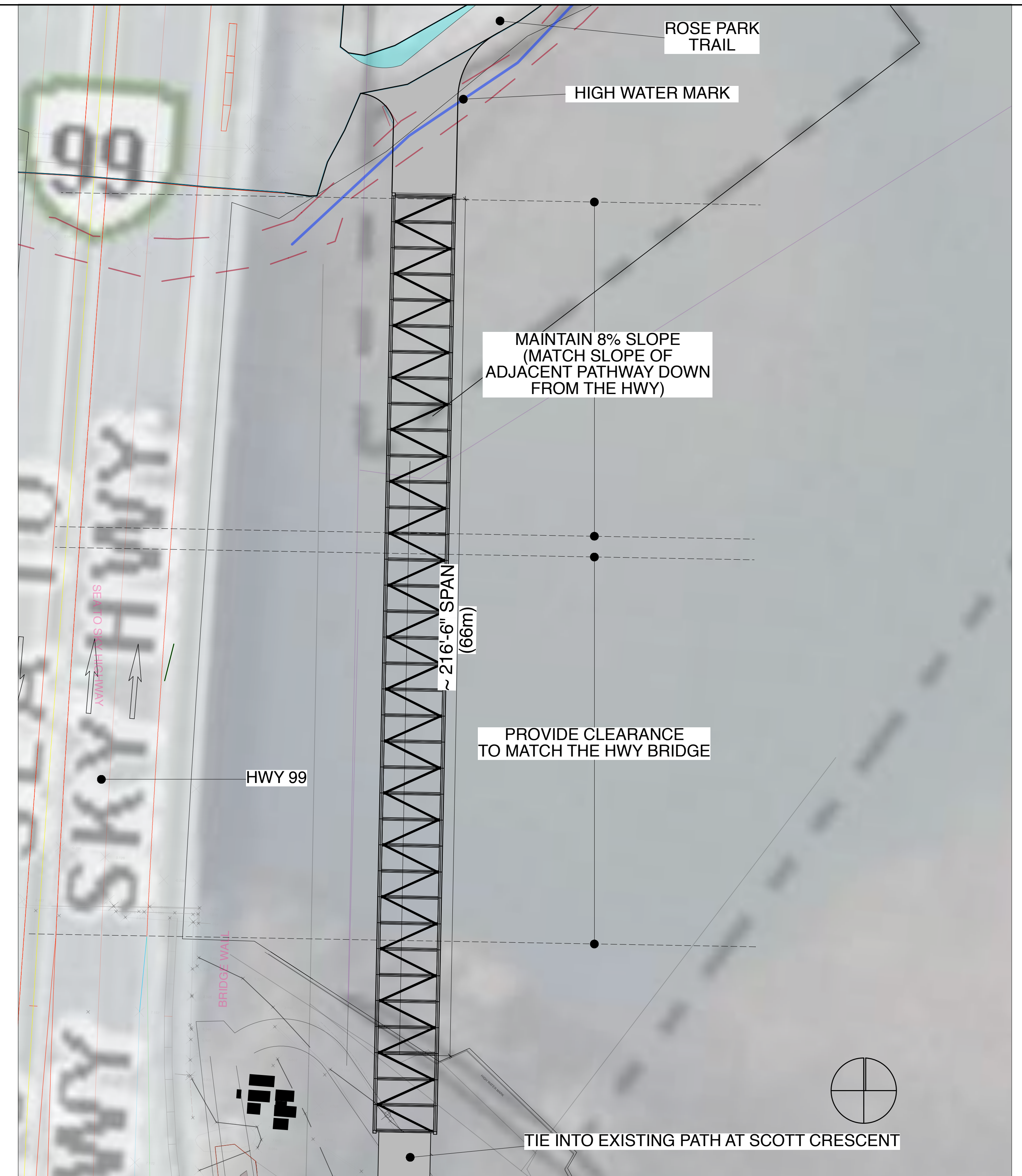
PROPOSED BRIDGE: CROSSING Scale : 1:200
