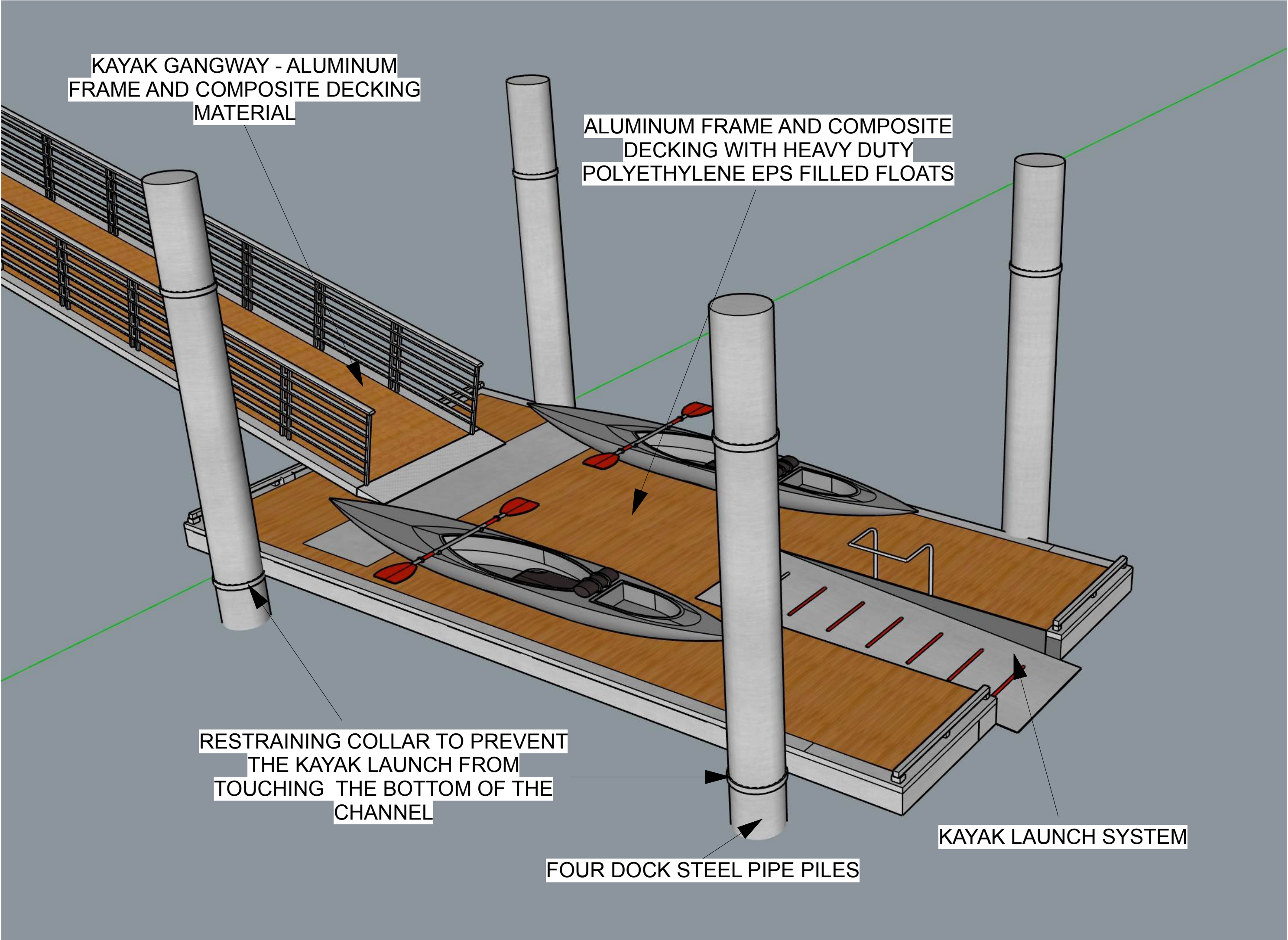
3D MODEL FOR KAYAK LAUNCH
